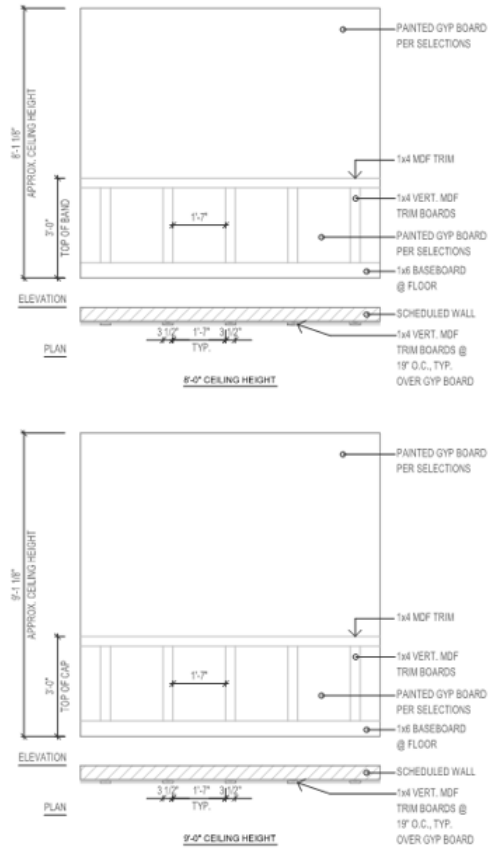
Clover Theme Wall Detail
