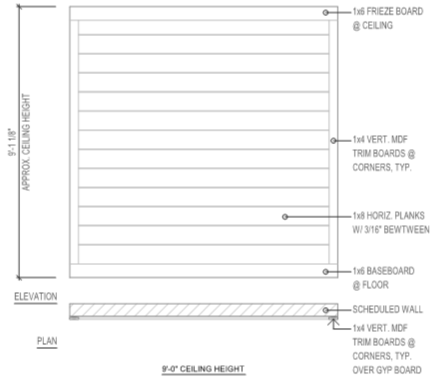
Magnolia Theme Wall Detail
