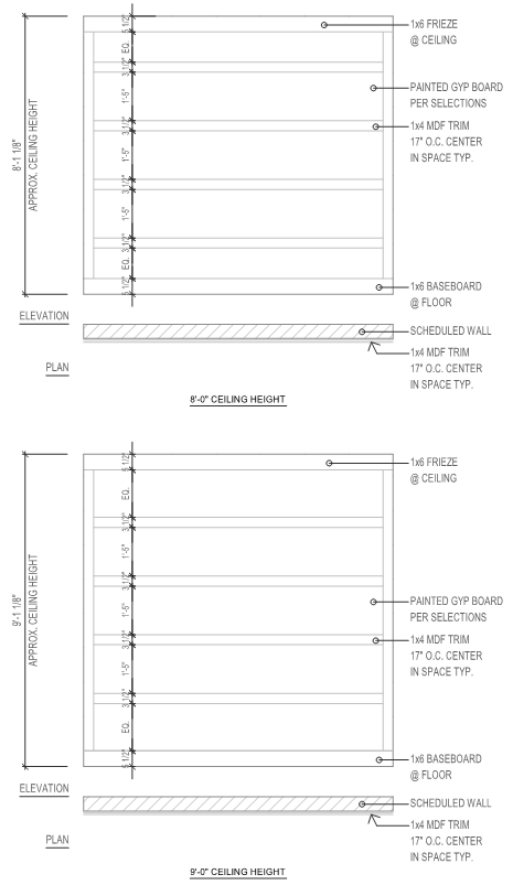
Willow Theme Wall Detail
